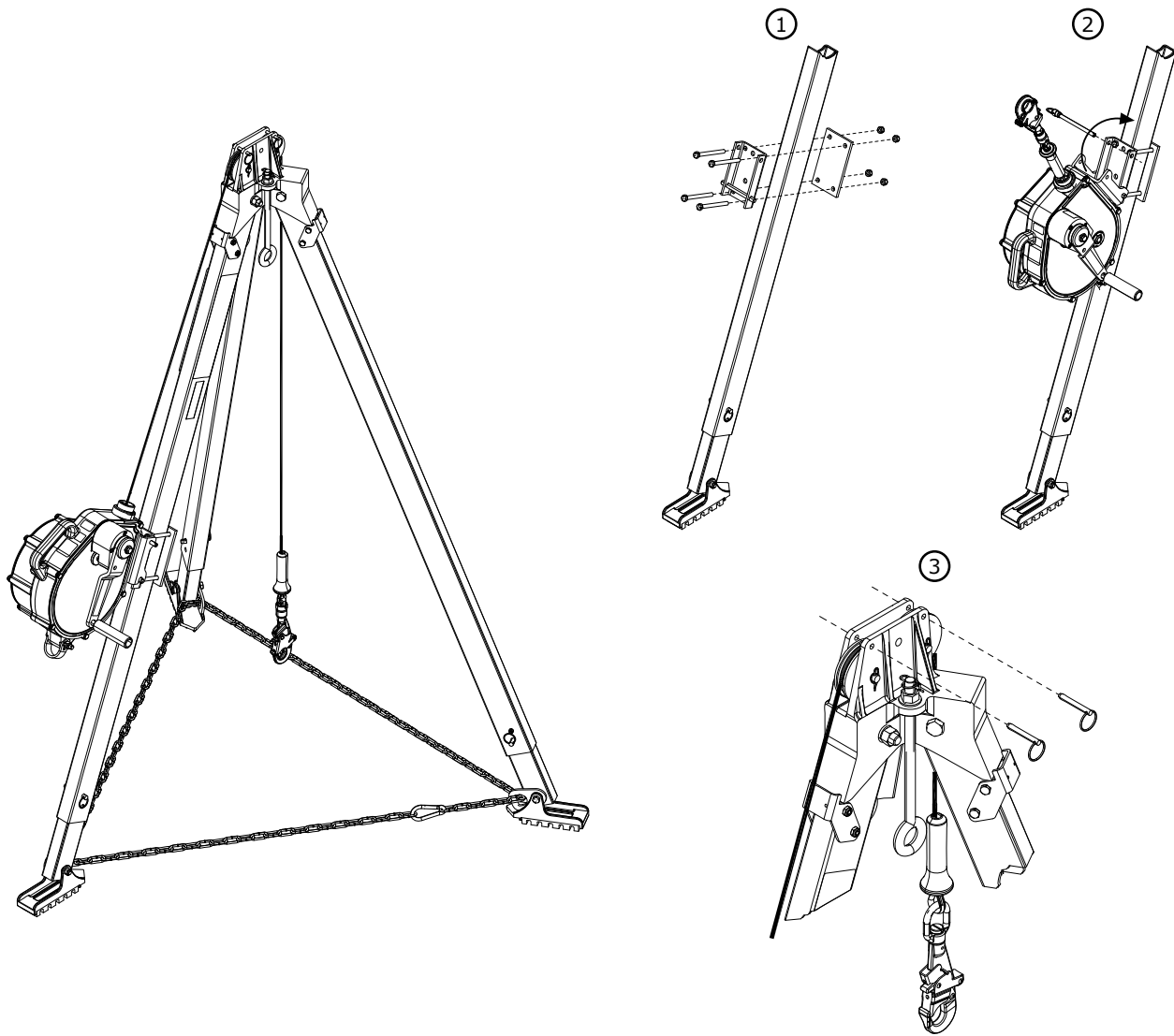
Figure 8 – Tripod Mounting
