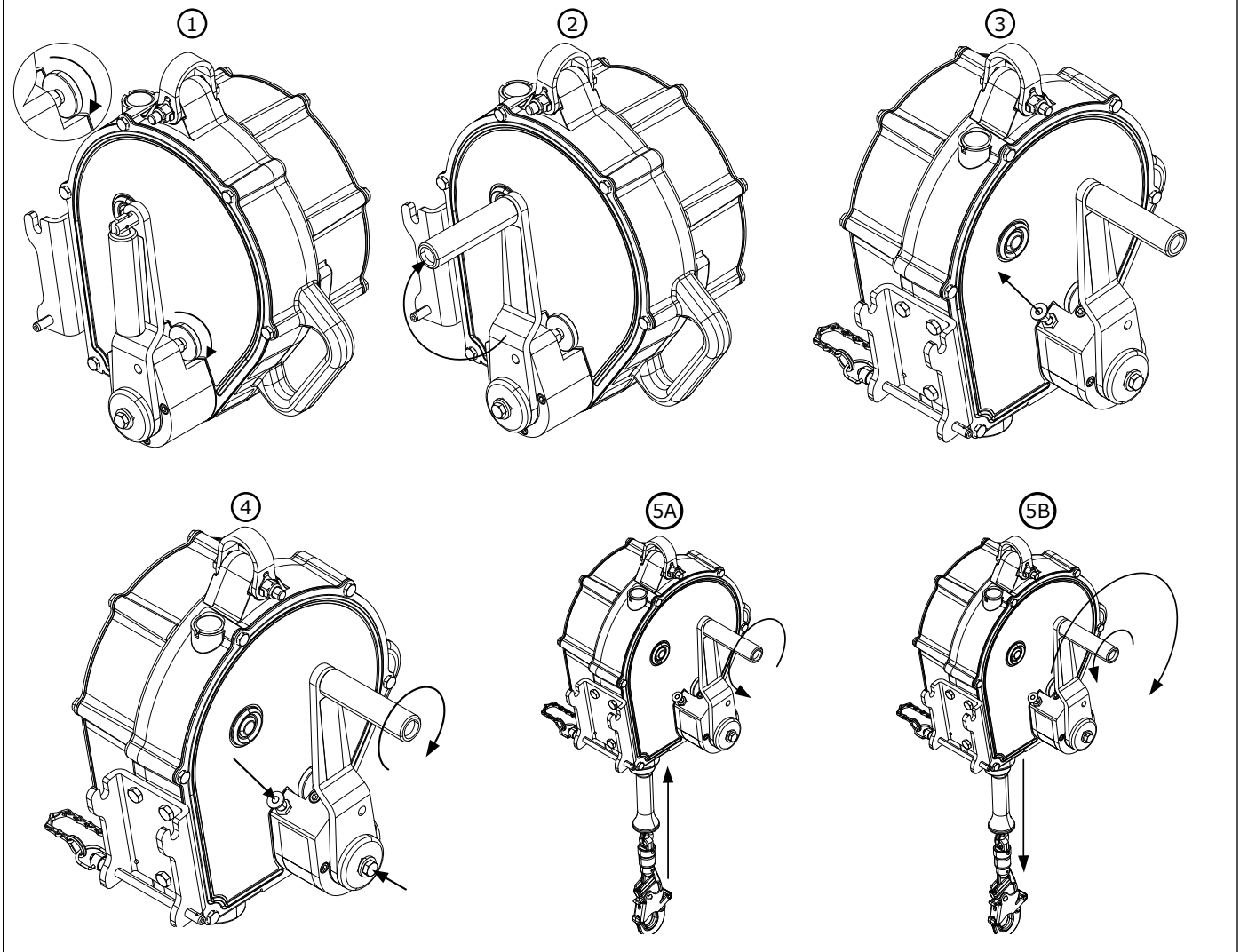
Figure 11 – Retrieval Operation
