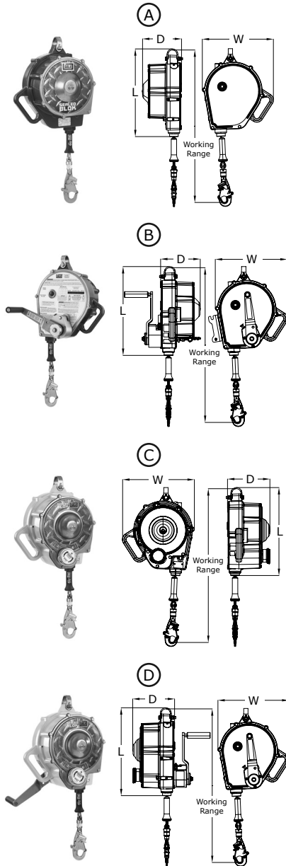
Figure 1 – Sealed-Blok™ Self-Retracting Lanyards with Fast-Line™ Cable Replacement
