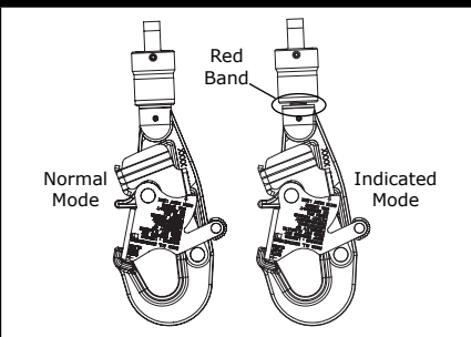
Diagram 2 – Impact Indicator
