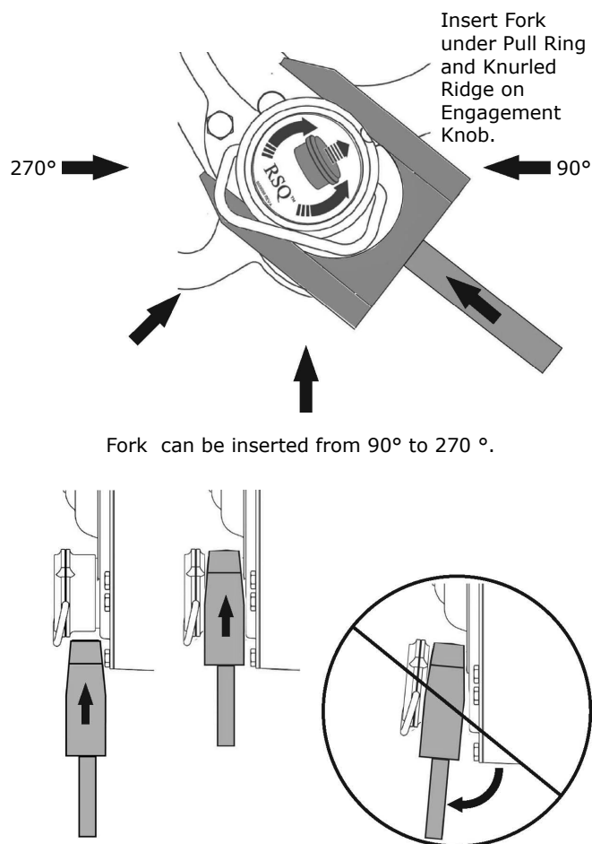
Figure 10 – Assisted Rescue Operation
