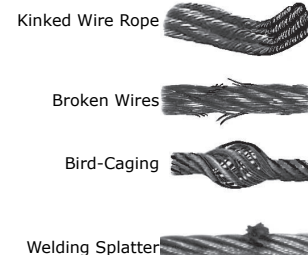
Diagram 3 – Wire Rope
