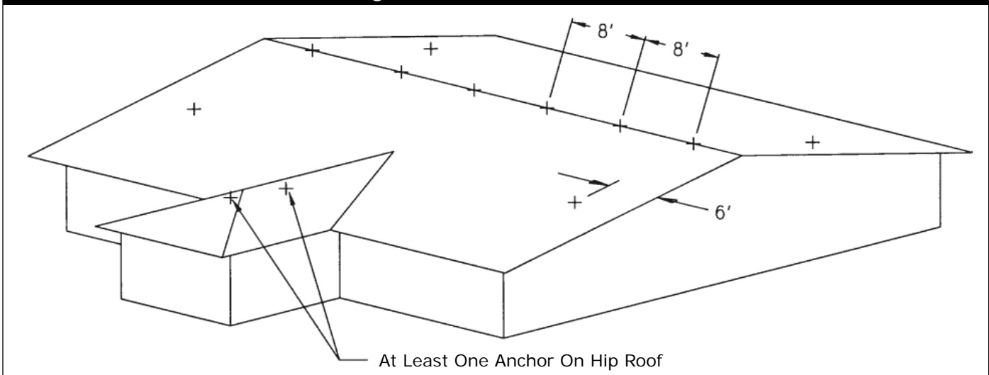
Figure 5 - Anchor Installation
