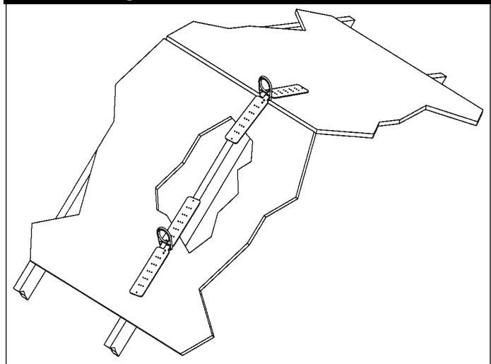
Figure 6 - Anchor Installation
