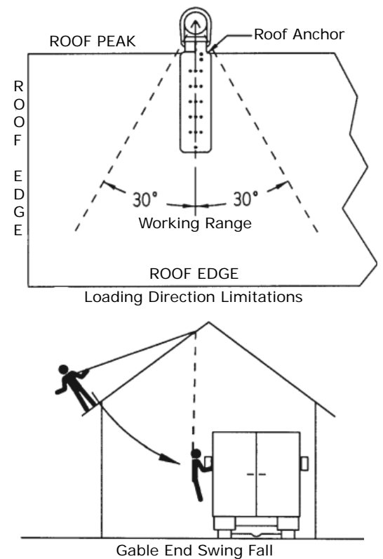
Figure 4 - Swing Fall
