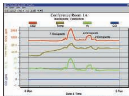
Easy-to-use TRAKPRO™ Data Analysis Software stores, organizes and reports test
