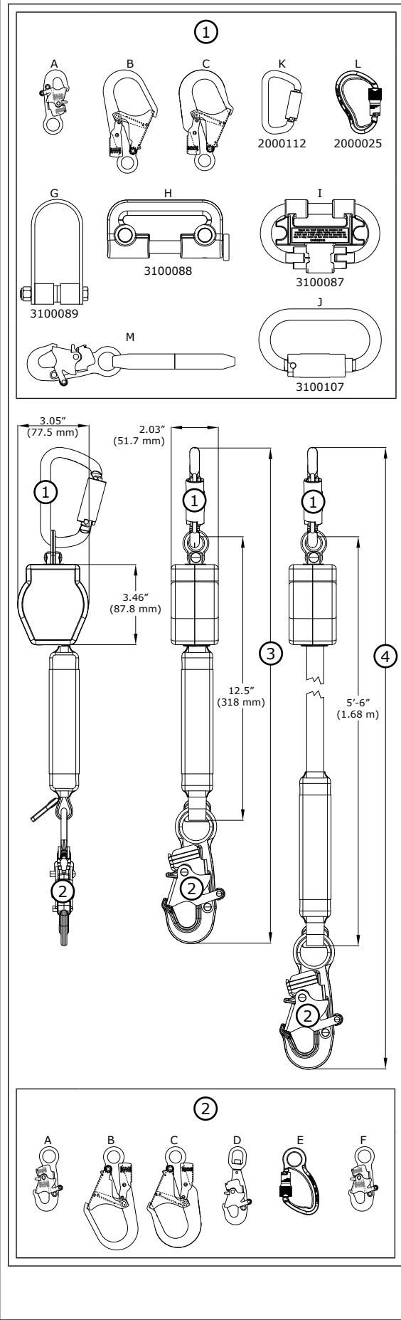
Figure 18 – Dimensions & End Connector Specifications
