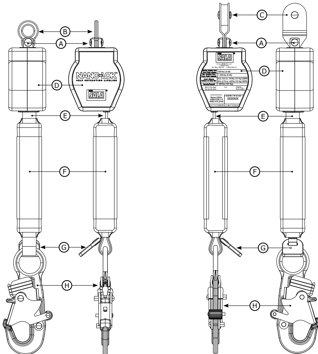
Figure 2 – Nano-Lok Self Retracting Lifeline (SRL) Components
