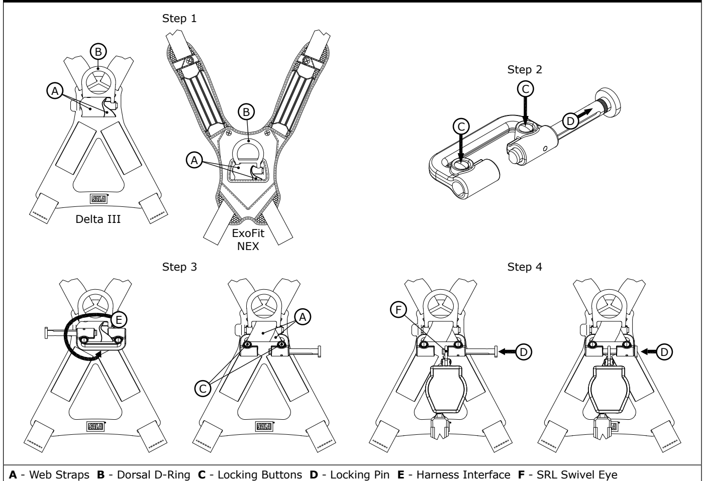
Figure 8 – Single SRL Harness Interface
