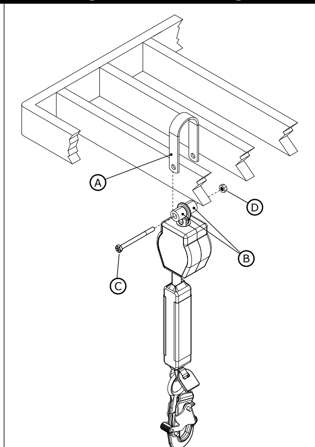
Figure 7 – Cab Mounting
