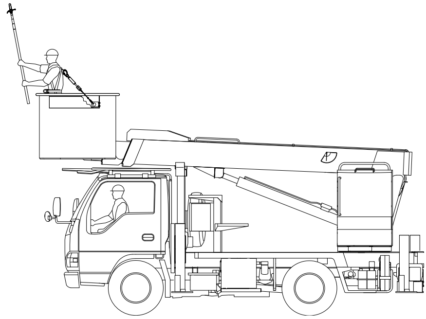
Model 3101375 Bucket Truck Application
