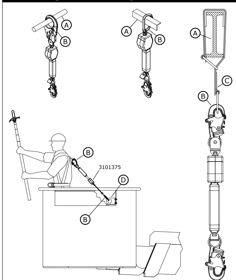
Figure 6 – Anchorage Connections
