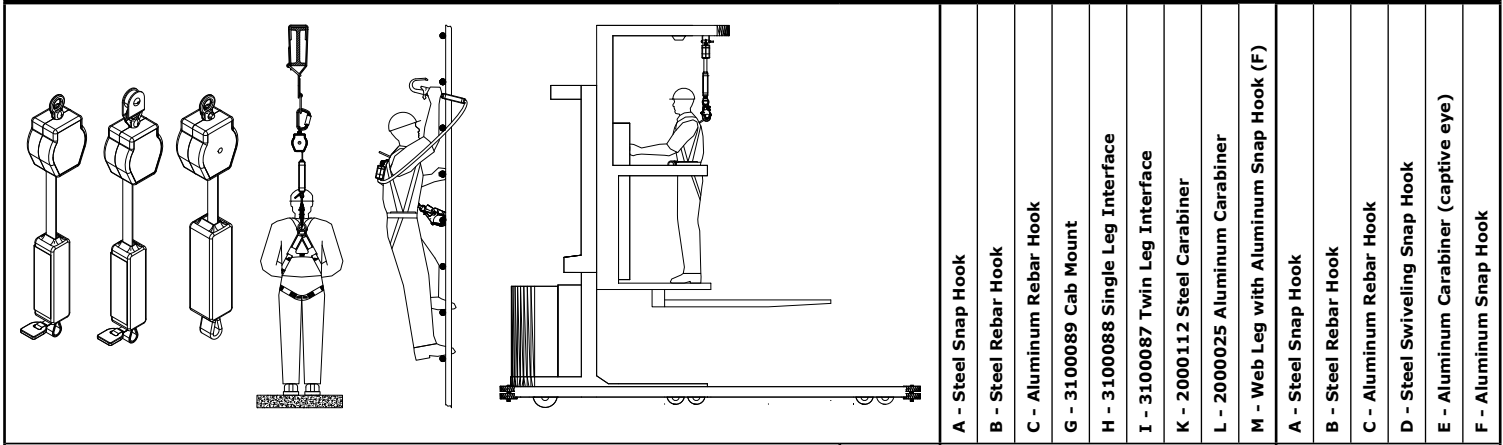
Figure 1 – Nano-Lok™ Self Retracting Lifeline Models
