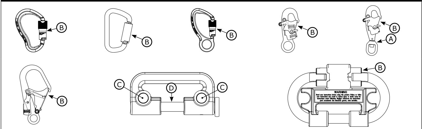
Figure 17 – End Connectors
